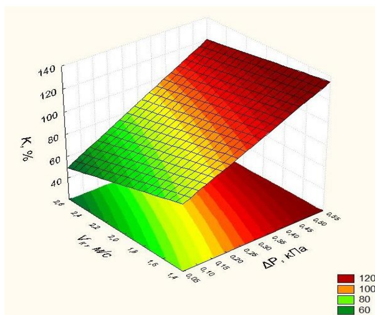
Fig. 1. The response surface and line of level output for cells filling factor of a seed disk.
